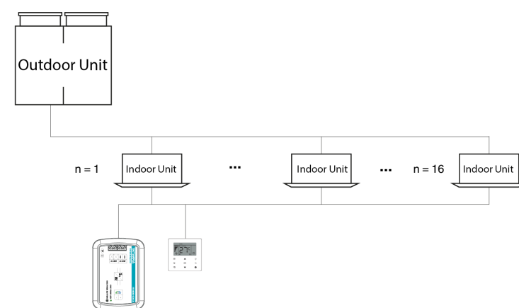
Gateway - Multi Indoor Unit + Remote Controller :
